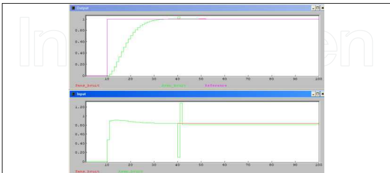
Fig. 11. Step response under and without disturbance.
