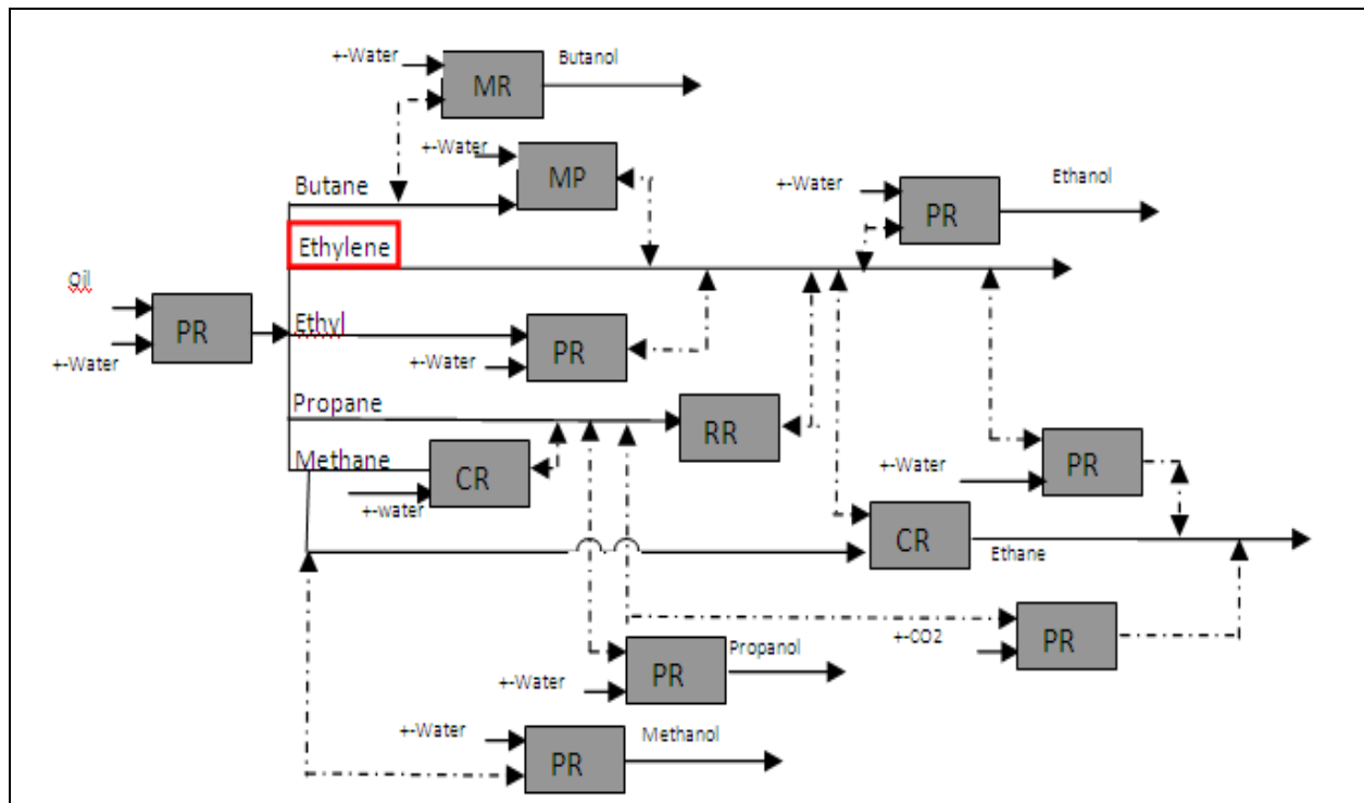
Fig. 1. Integration of Pyrolysis reactor into a petrochemical plant
