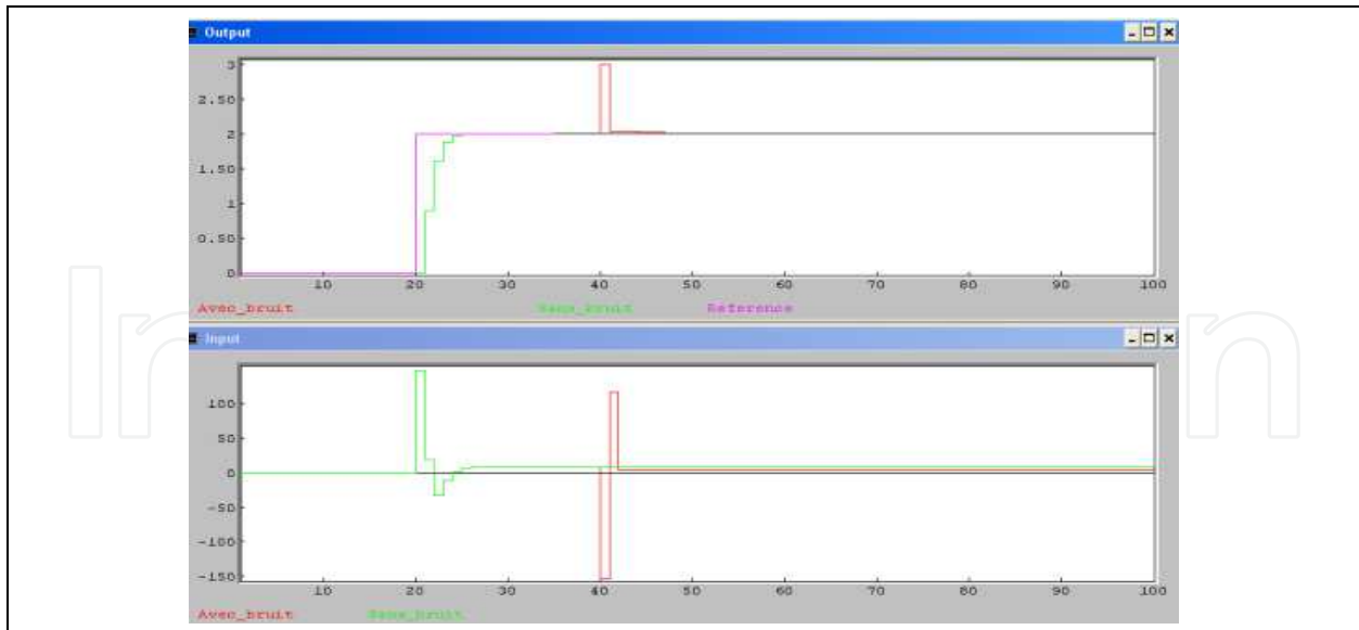
Fig. 14. Step response under and without disturbance.
