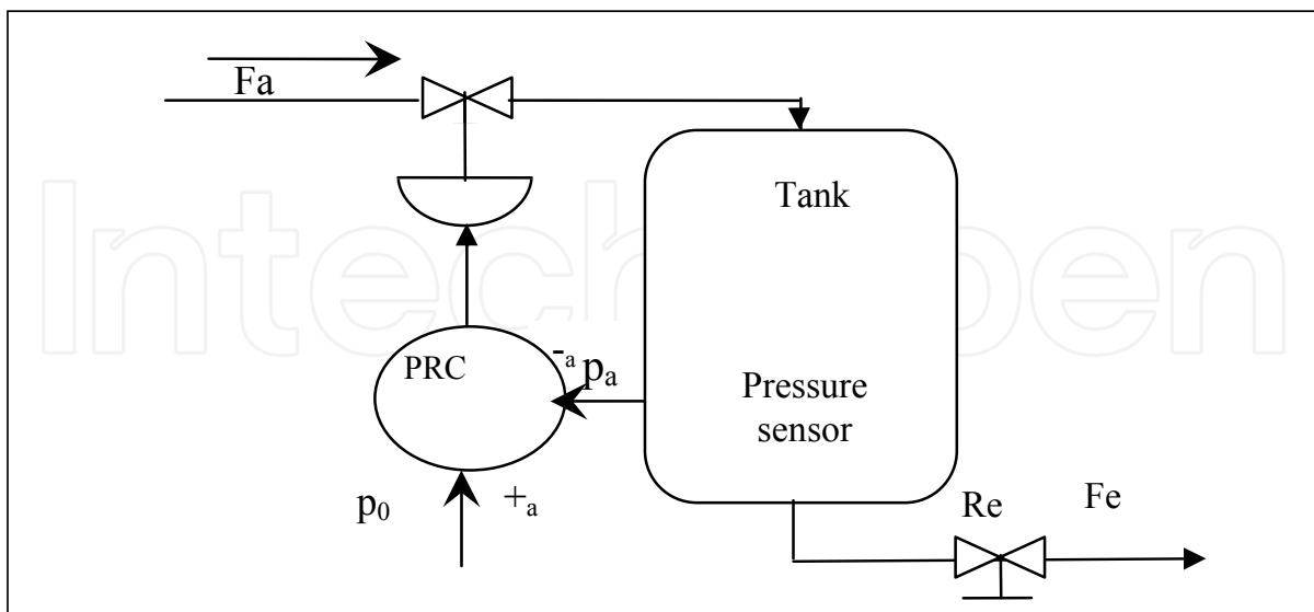
Fig. 8. Pressure control
