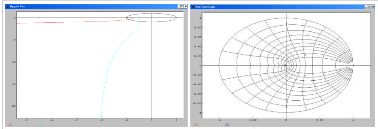
Fig. 9. Nyquist diagram and poles in closed loop.
