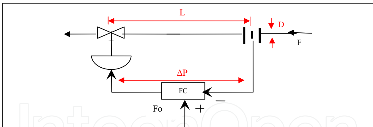
Fig. 3. Flow controller
