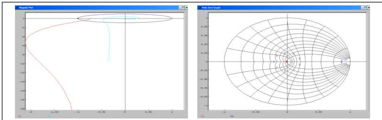
Fig. 13. Nyquist diagram and closed-loop poles.
