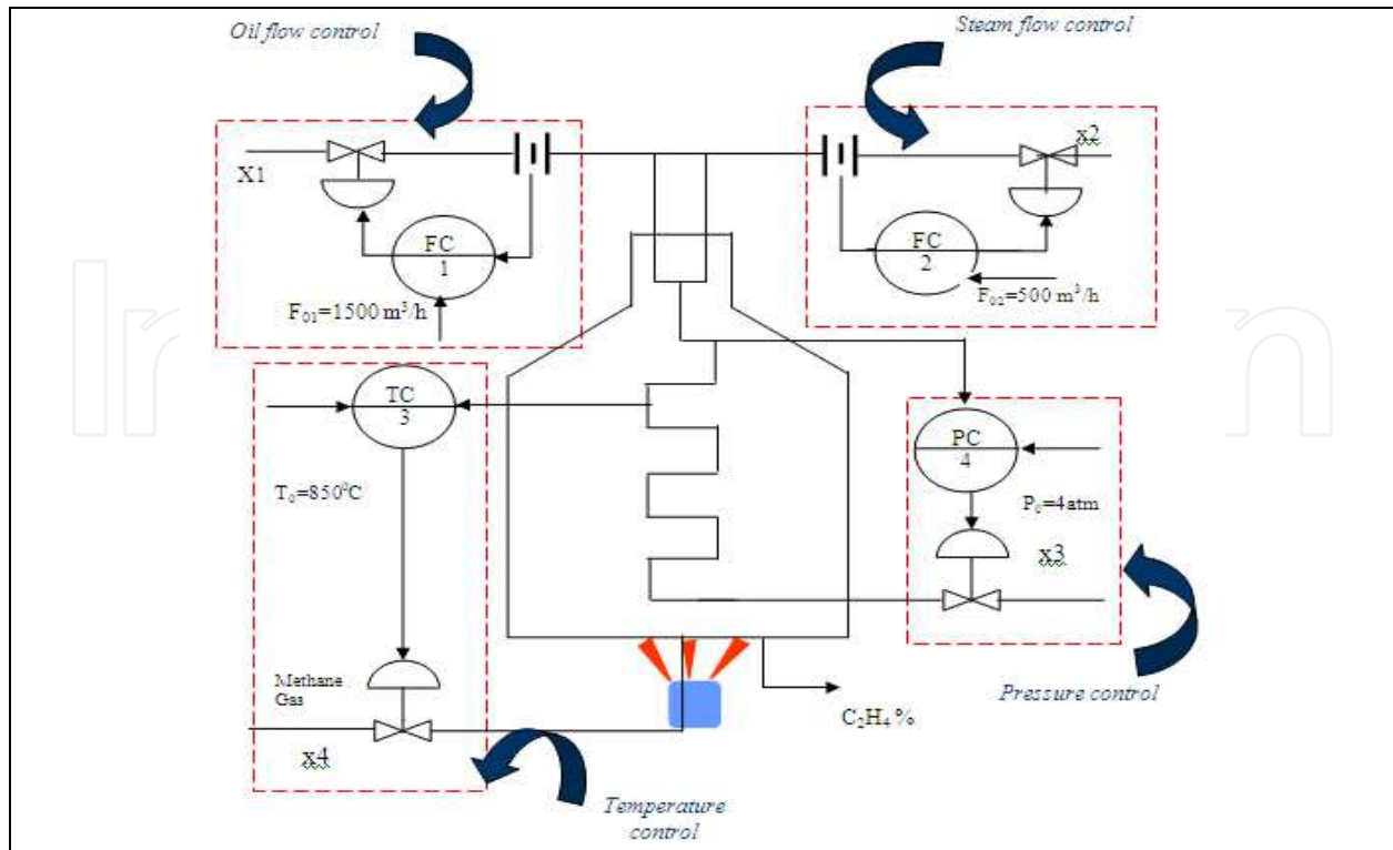
Fig. 2. Controller loops that govern the pyrolysis reactor.
