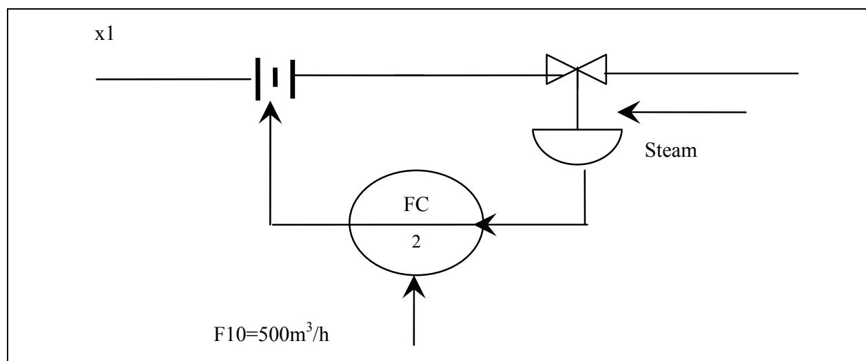
Fig. 6. Control of steam flow.
