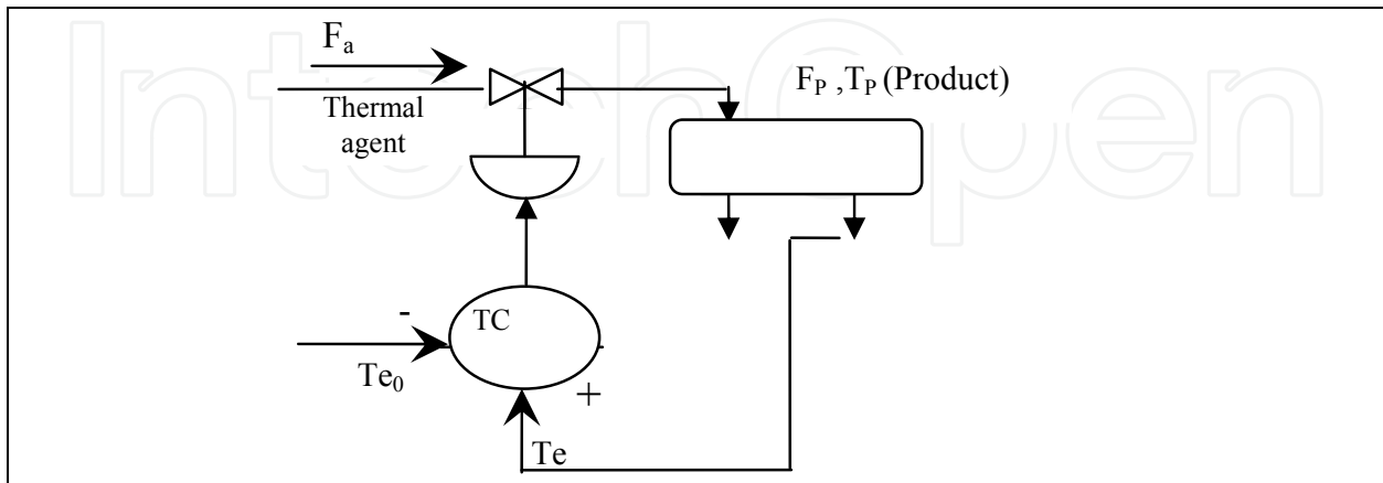
Fig. 12. Temperature control
