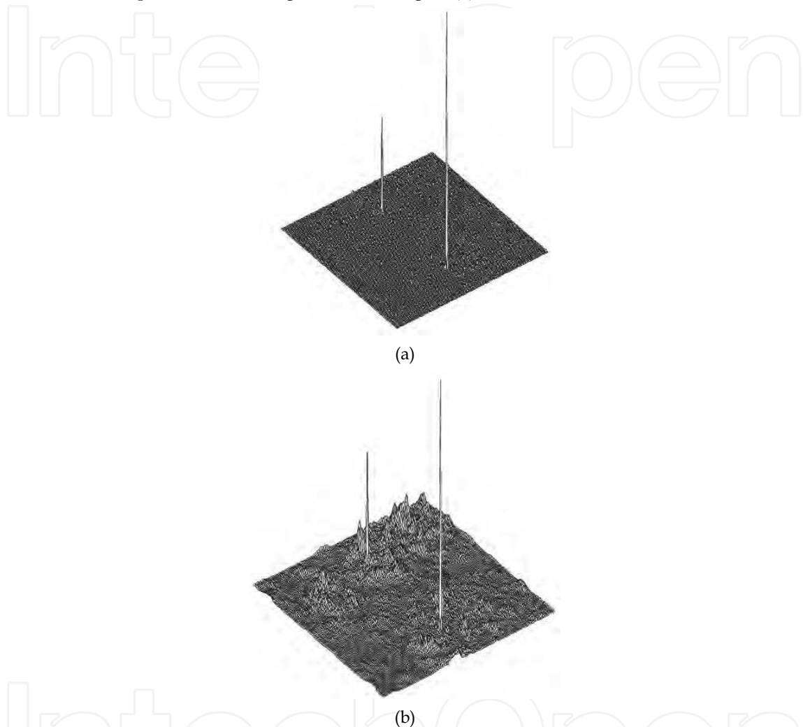
Fig. 14. Computer simulation results obtained for the input scene in Fig. 13 (a) with: (a) binary JTC, (b) fringe-adjusted JTC.
