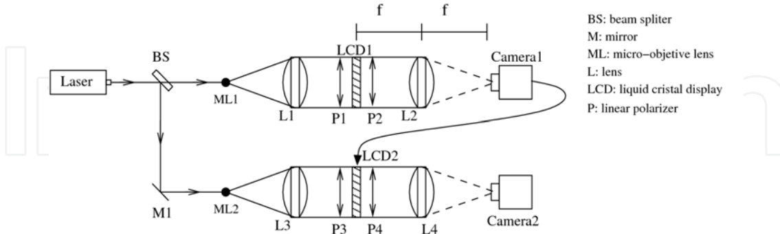
Fig. 10. Block diagram of the classical JTC.
