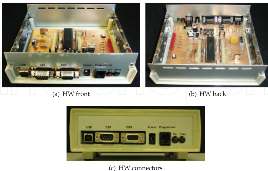
Fig. 2. Hardware Design
