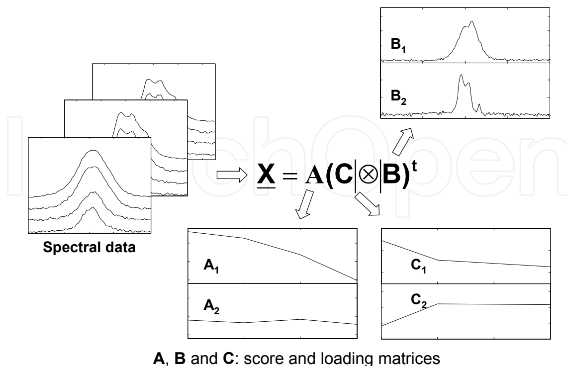
Fig. 2. Schematic illustration of PARAFAC trilinear model.
