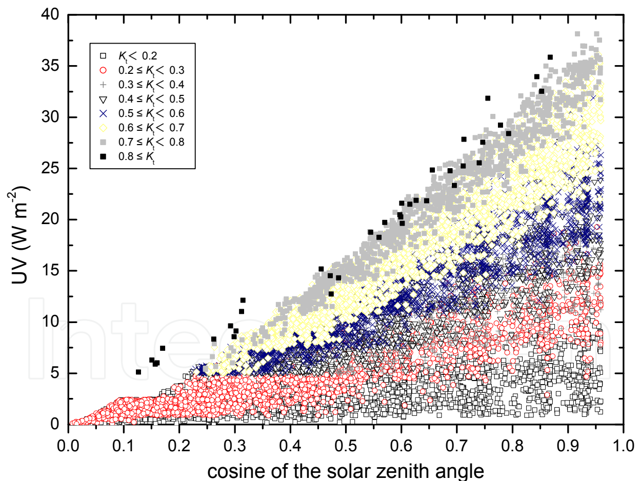
Fig. 4. UV as a function of the cosine of the solar zenith angle at different K_t . Different clearness index ( K_t ) values are represented by different colours. The values of UV radiation within a narrow range of clearness index values increase almost exponentially with the cosine of the solar zenith angle.
