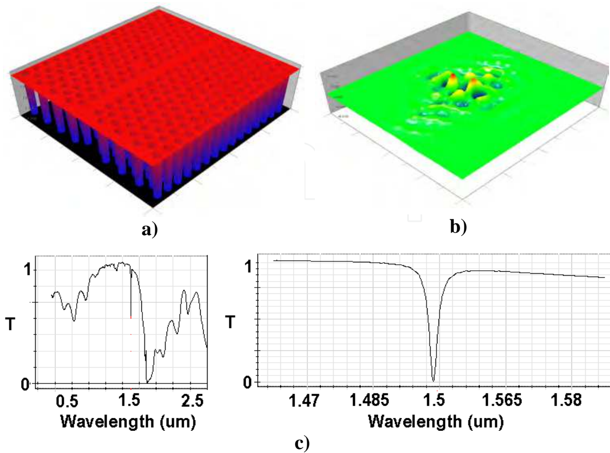
Fig. 15. a) Dielectric constant structure of a cavity coupled to a waveguide on a 2D triangular lattice of holes in lithium niobate; b) DFT of H_{-1} ; c) Transmission diagram over wavelength and detail of the resonance and surrounding wavelengths.
