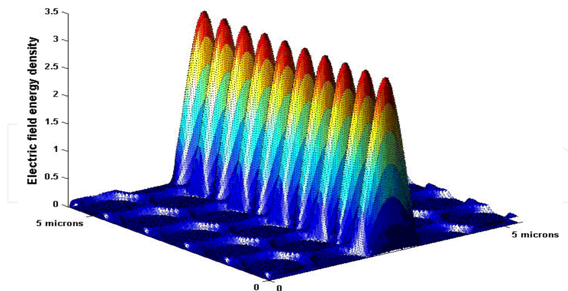
Fig. 10. Electric field energy density confined within the photonic crystal waveguide.
