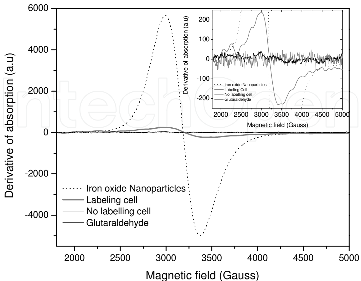
Fig. 4. EPR spectra, showing the resonance absorption curve of the superparamagnetic nanoparticles, labelled cells (CD133 + ), unlabelled cells (CD133 - ) and glutaraldehyde 0,5% fixative. The spectra are shown in the inset.
