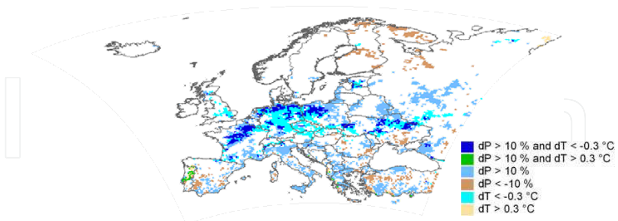
Fig. 6. The regions with the largest effects of forest cover increase on temperature and precipitation (dT: temperature change, dP: precipitation change)
