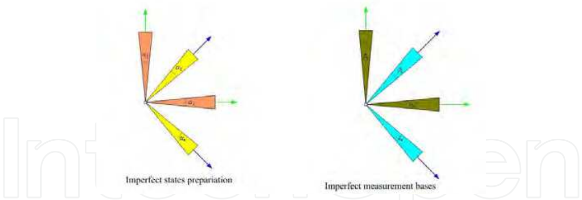
Fig. 5. The most general imperfect states preparation and measurement in practical QKD experimental realization.
