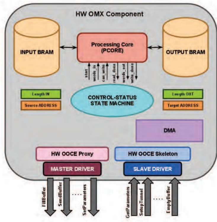
Fig. 10. Hw OMX Component structure
