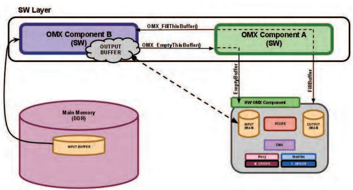
Fig. 15. Software-to-Hardware communication model.
