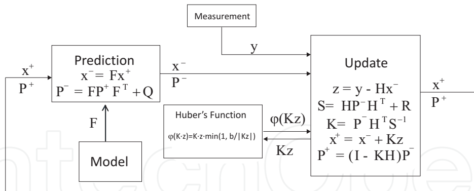
Fig. 14. Block diagram of the robust Kalman filter
