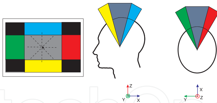
Fig. 9. Control space of joystick mode
