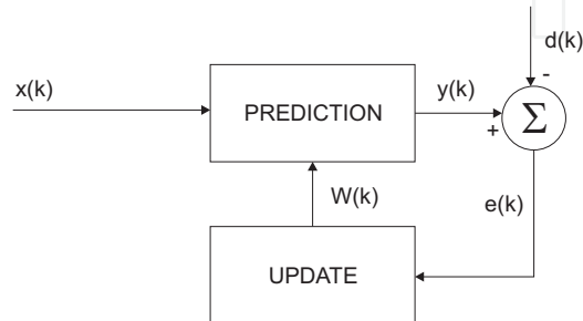
Fig. 10. Block diagram of adaptive filtering implementation
