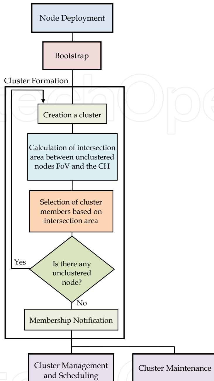
Fig. 2. Clustering Procedure.
