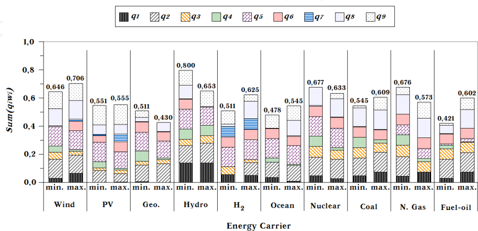
Fig. 18. Maximum and minimum values range of sustainability index for each energy carrier system - Case Scenario 8 (Highest weighting factor for selected indicators: q_1, q_2, q_5, q_8, q_9 ).
