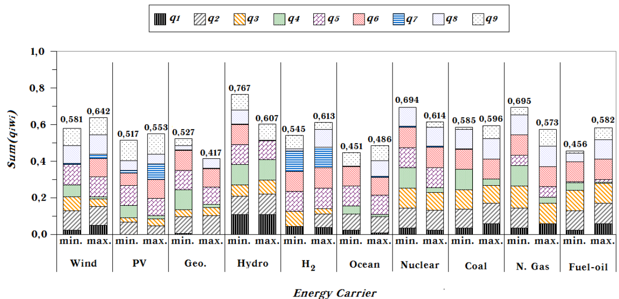
Fig. 11. Maximum and minimum values range of sustainability index for each energy carrier system - Case Scenario 1 (Equal weighting factors for indicators).
