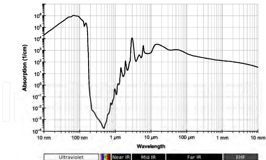
Fig. 11. The absorption spectrum of ultrapure water (Querry and al., 1998)
