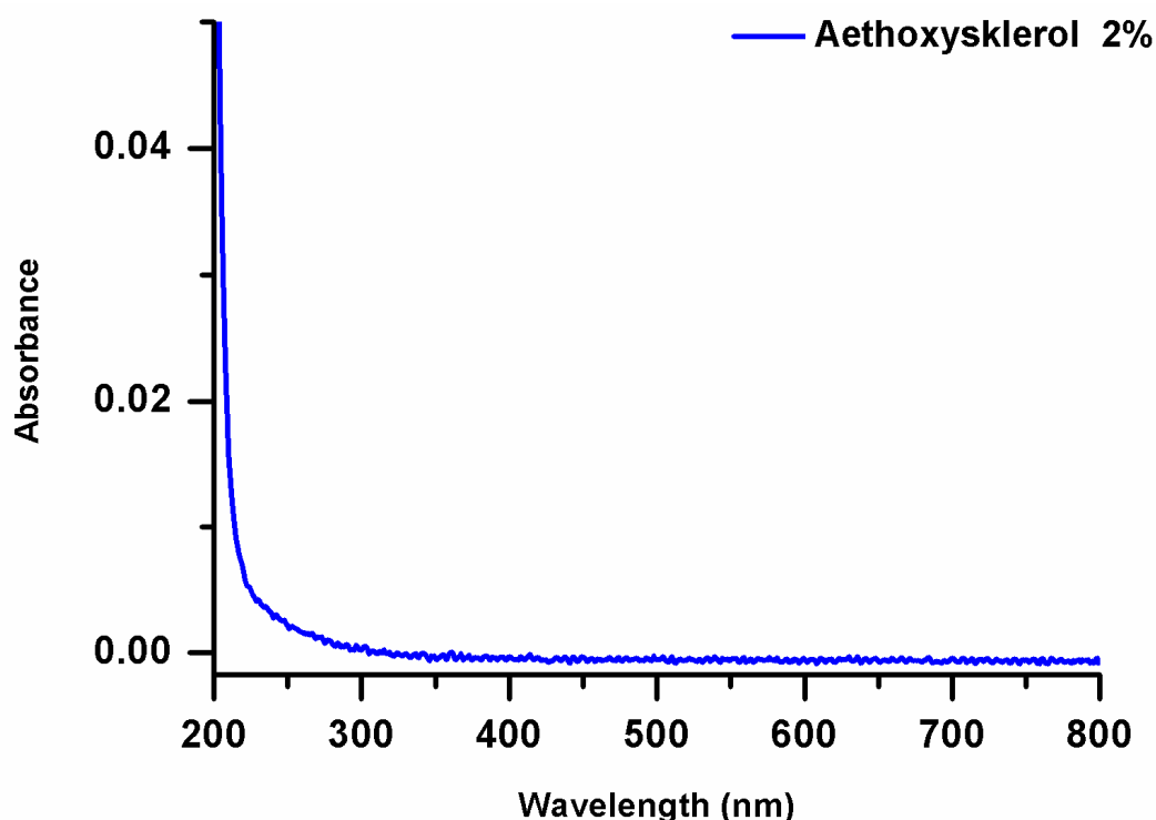
Fig. 7. UV-VIS absorption spectrum of Aethoxysklerol 2%
