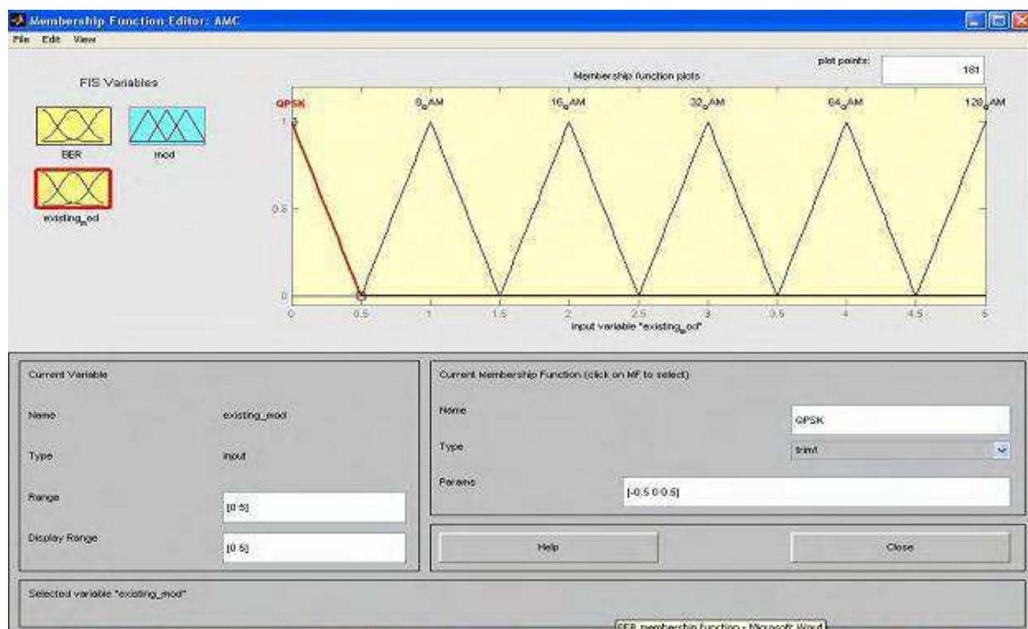
Fig. 13. Present mod membership functions
