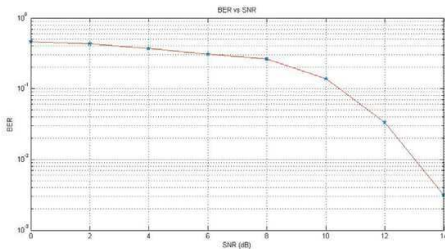
Fig. 8. Bit error rate of OFDM system
