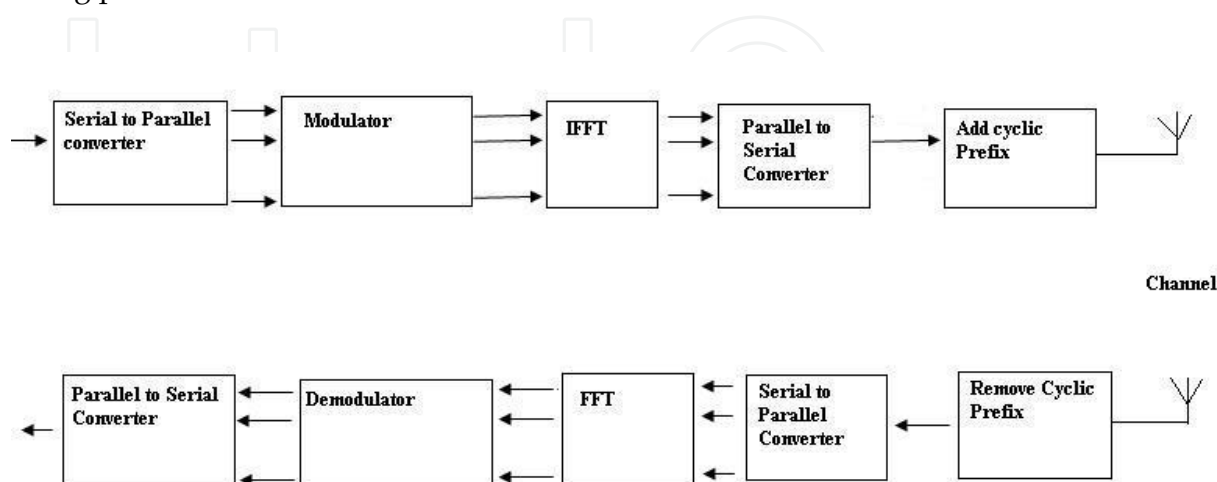
Fig. 1. OFDM system
