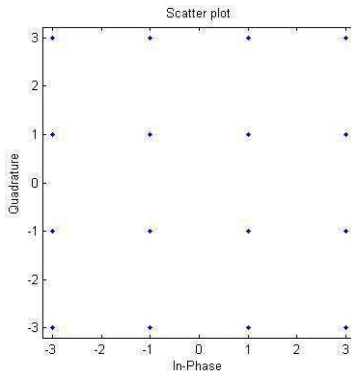
Fig. 4. Constellation ordering of 16-QAM modulator
