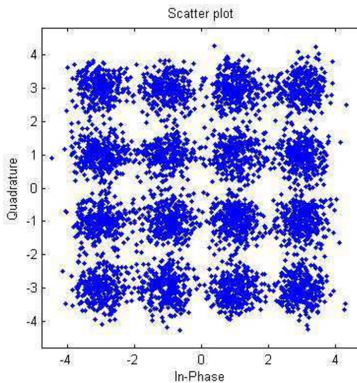
Fig. 7. Constellation ordering at receiver
