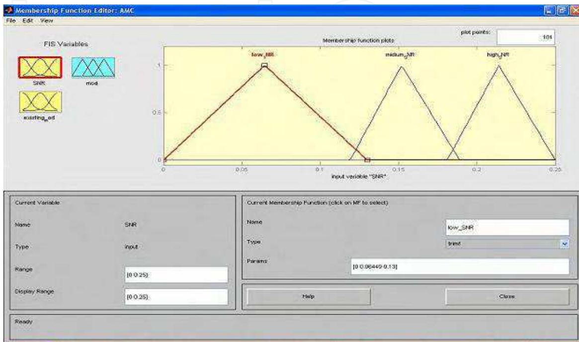
Fig. 12. SNR membership functions
