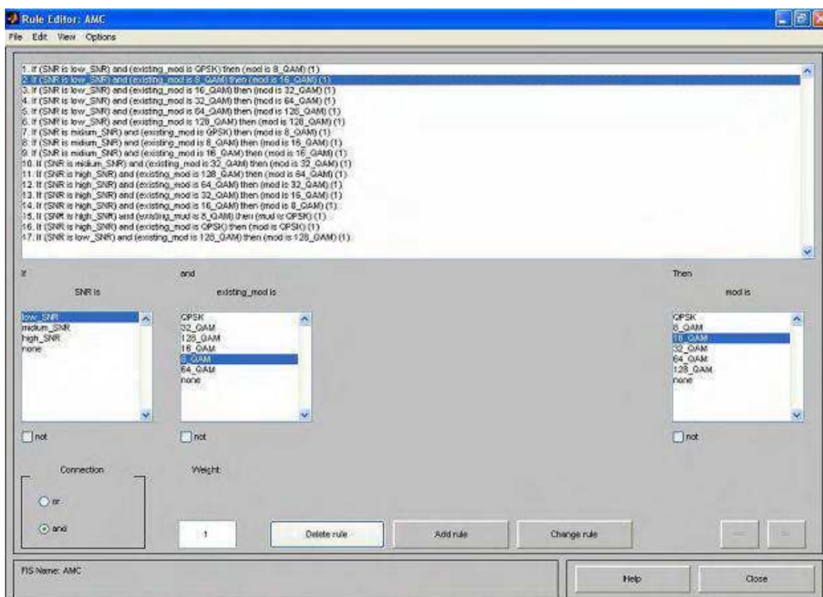
Fig. 15. Rules editor
