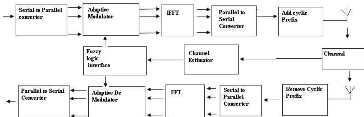
Fig. 9. Adaptive modulated OFDM system
