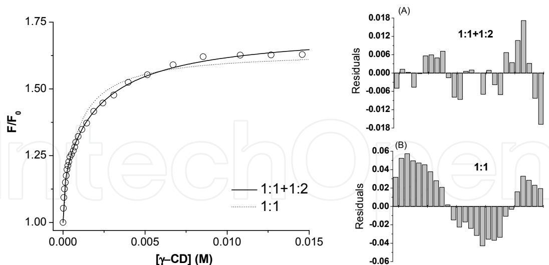
Fig. 4. Normalized experimental data fits with eqs. 7 (solid line) and 3 (dotted line) for the determination of the stoichiometry of the DEAC- \gamma -CD complex. Inset: The distribution of the residuals for the (A) 1:1+1:2 and (B) 1:1 fits.
