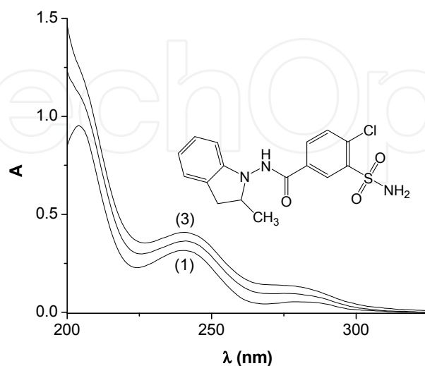
Fig. 5. The absorption spectrum of indapamide ( 10^{-5} M in methanol:water 1:9 v:v) in absence (1) and presence (2, 3) of increasing concentrations of 2-HP- \beta -CD (up to 2 \times 10^{-2} M).
