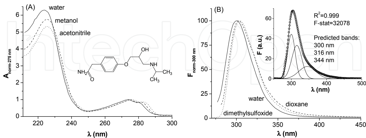
Fig. 8. Absorption (A) and fluorescence (B) spectra of atenolol in different solvents. Inset: Deconvolution of the fluorescence spectrum of atenolol in dimethylformamide. \lambda_{ex} = 275 \text{ nm} .
