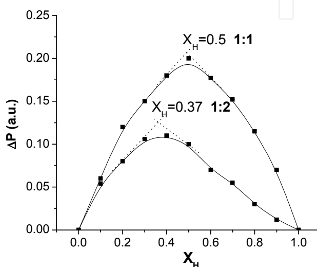
Fig. 1. Typical Job's plots for 1:1 and 1:2 complexes.
