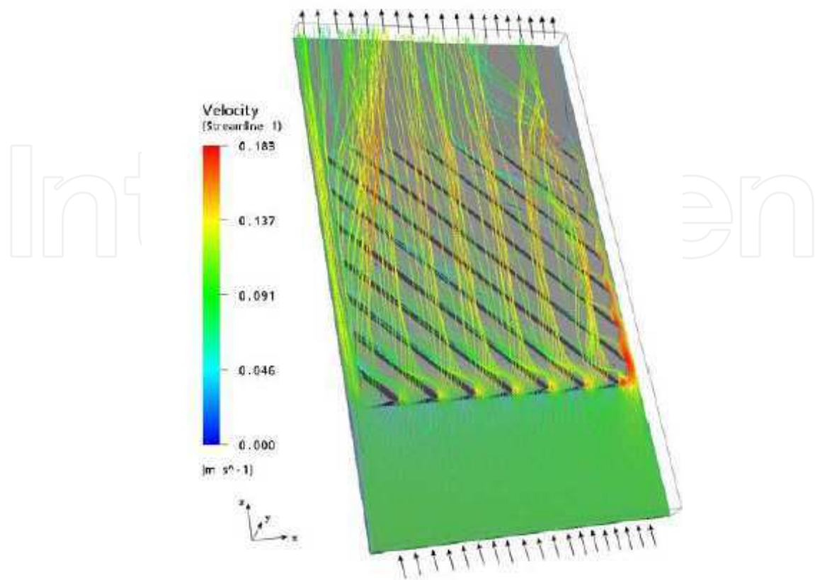
Fig. 11A. Typical flow pattern for the: a) simple channel, CFD results, Re=900 .
