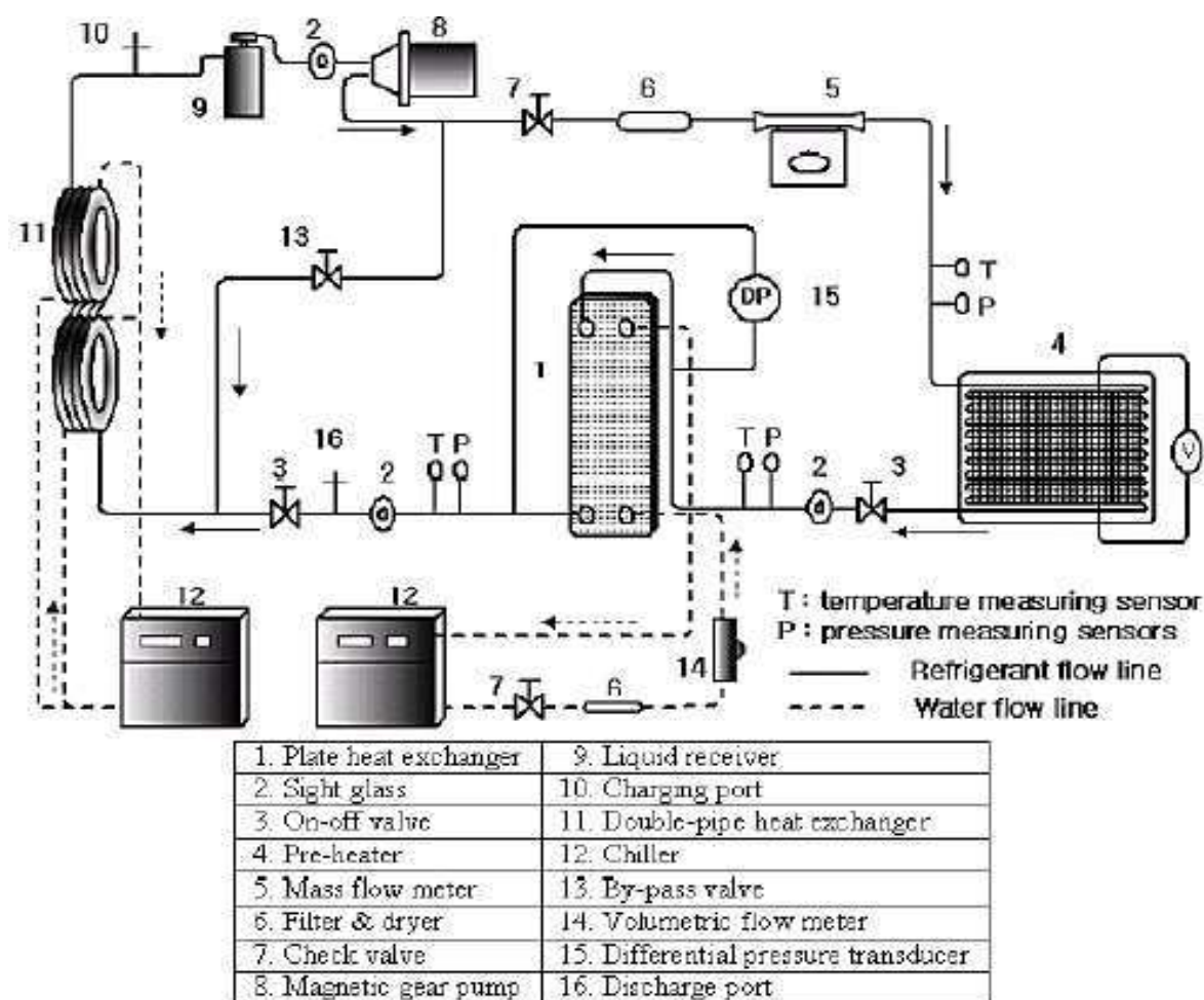
Fig. 1. Schematic diagram of the experimental system.
