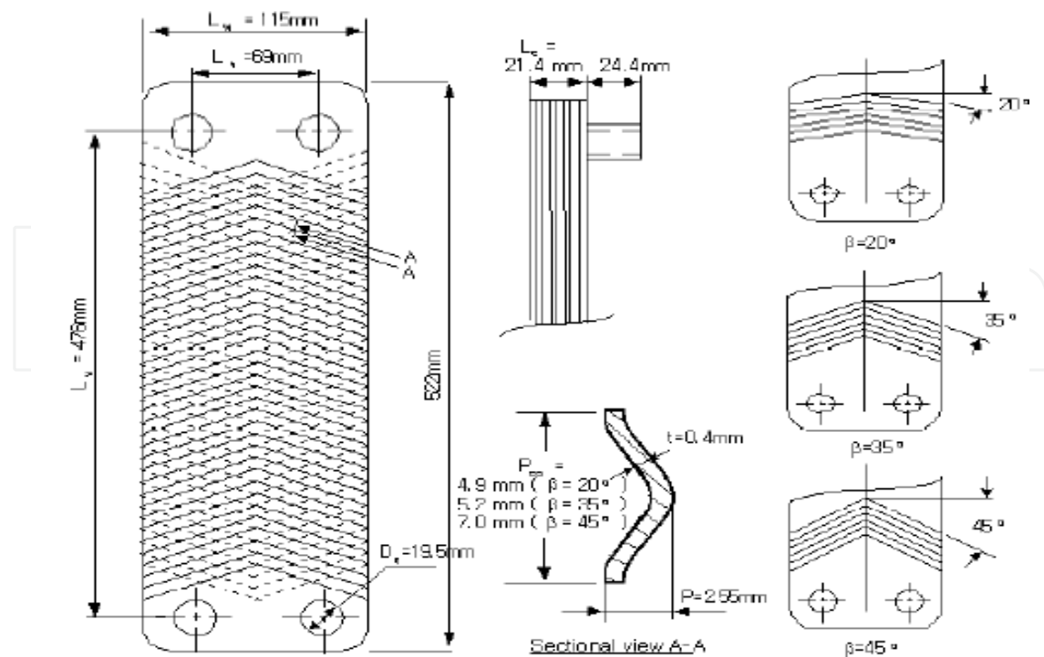
Fig. 2. Dimensions of the brazed plate heat exchangers.
