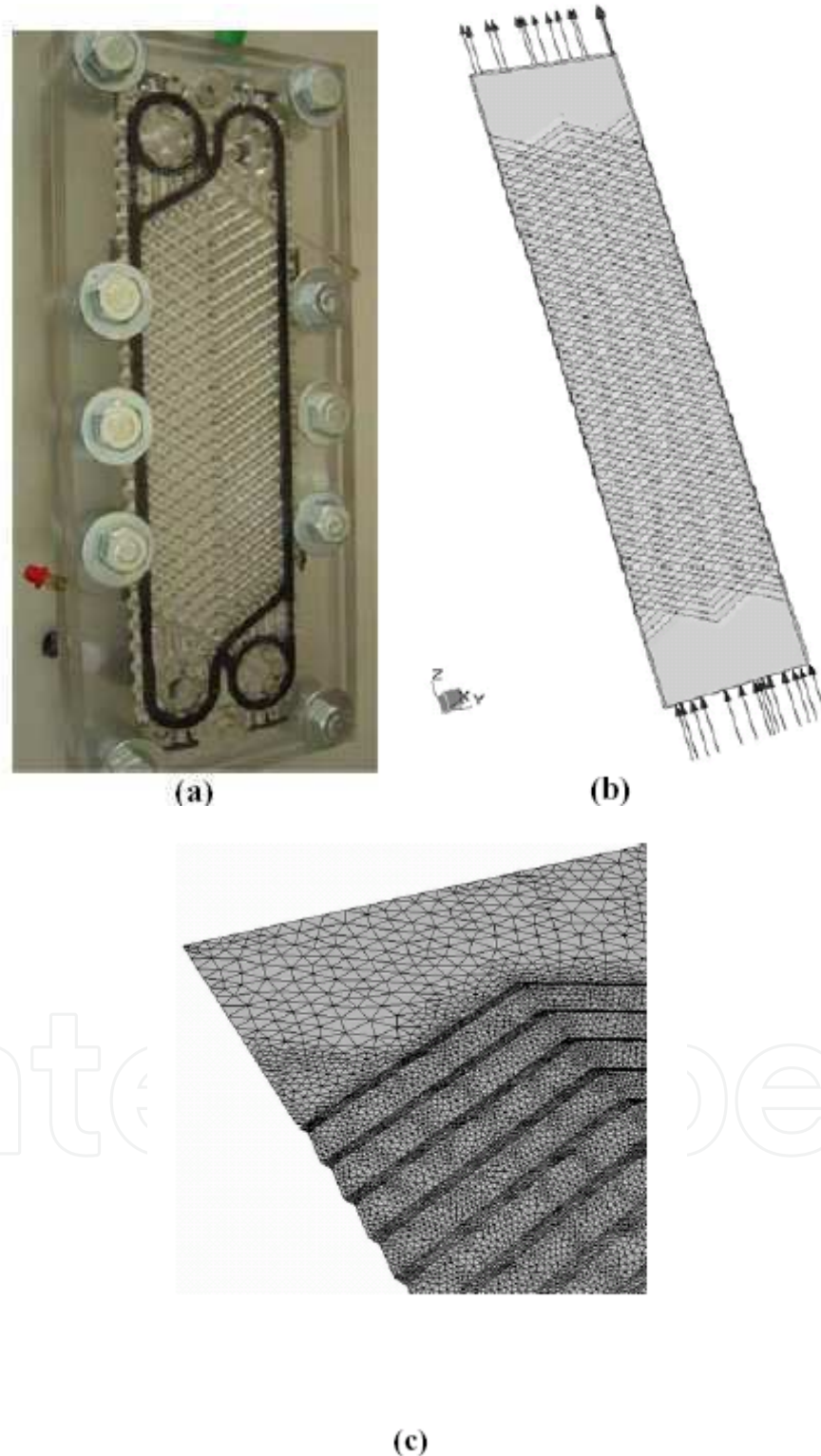
Fig. 16. (a) Module of a corrugated plate exchanger; (b) The CFD model and (c) Detail of the grid distribution over the corrugated wall.
