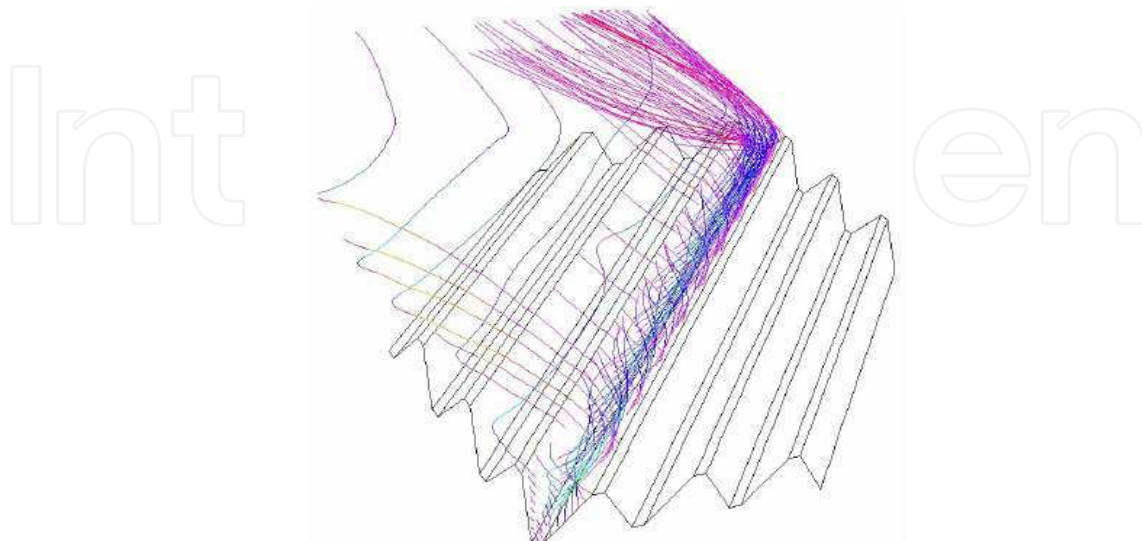
Fig. 12. Swirling flow inside a furrow; Re=900 .
