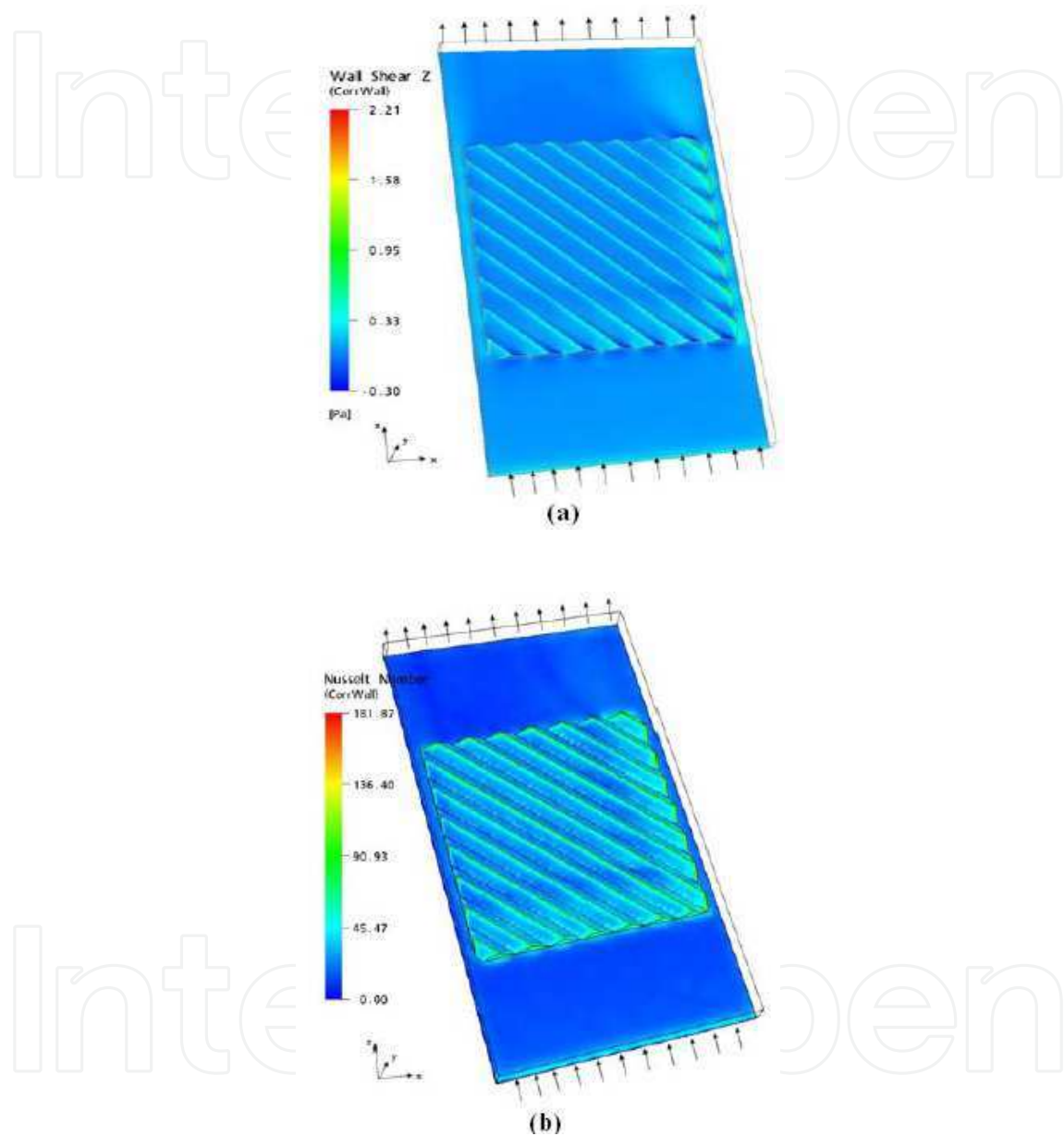
Fig. 13. Typical results of the CFD simulation for Re=900; distributions of: (a) z-shear stress component, (b) local Nusselt number.
