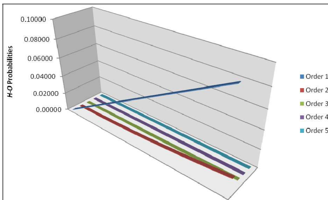
Fig. 2. Expanding Event-Spacetime, [P(E) = 0.10]
