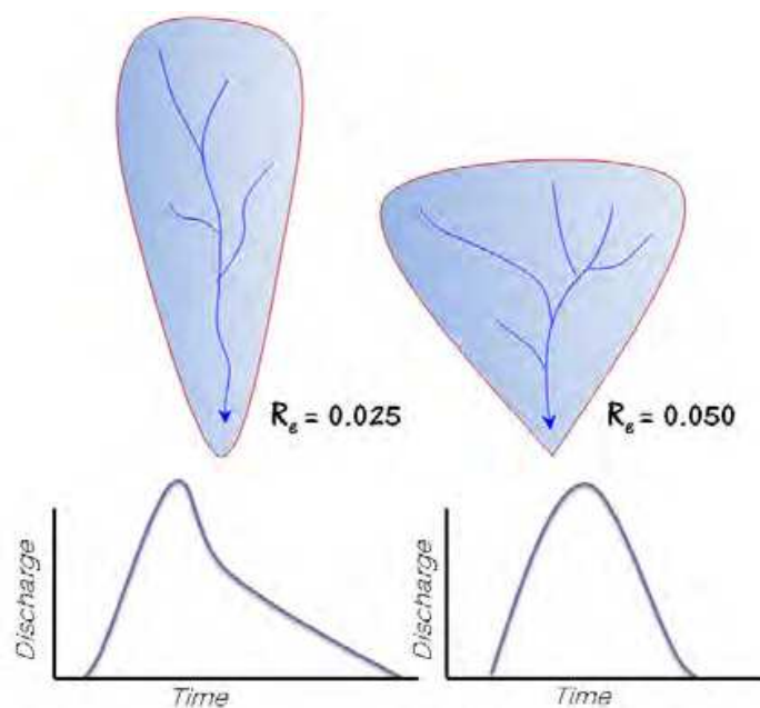
Fig. 9. Representation for two basins with different elongation ratio.
