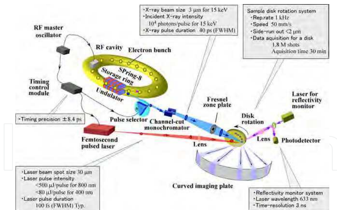
Fig. 2. Experimental setup for taking a snapshot of X-ray diffraction profile of optical phase-change materials.
