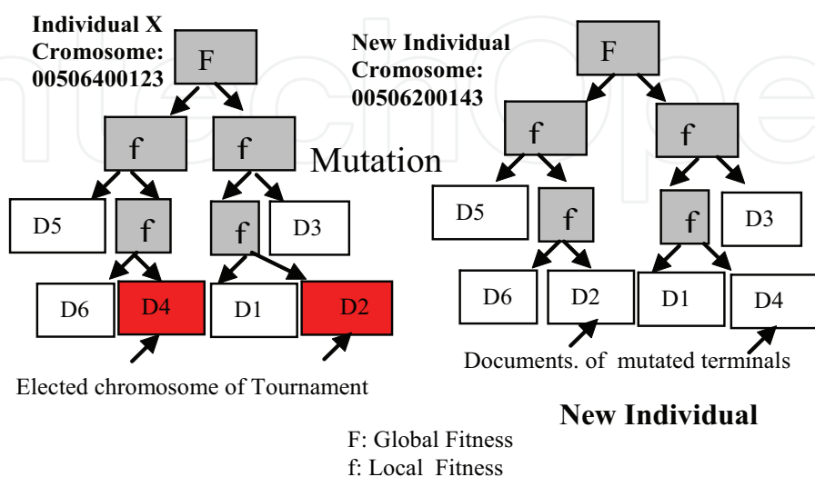
Fig. 4. Basic mutation operator applied to terminal
