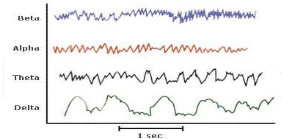
Fig. 3. Typical normal brain waves in the EEG
