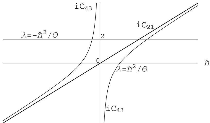
Fig. 1. The commutators i c_{21} and i c_{43} of the phase space as functions of \hbar .
