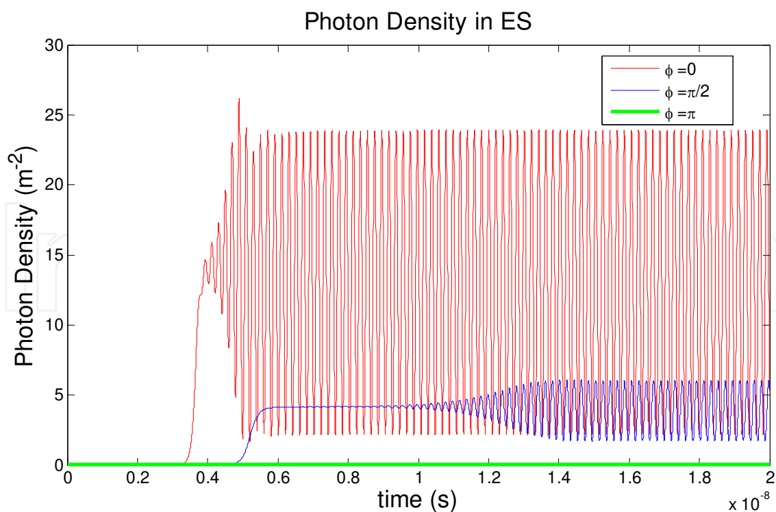
Fig. 7. Time series of ES photon density at three phase values when J_{ct}=1.5 J_{th} , \tau = 100ps , \alpha=2 and \gamma=0.025e12 .
