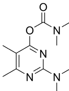
Fig. 2. Chemical structure of pirimicarb. Source: INCHEM ( www.inchem.org )
