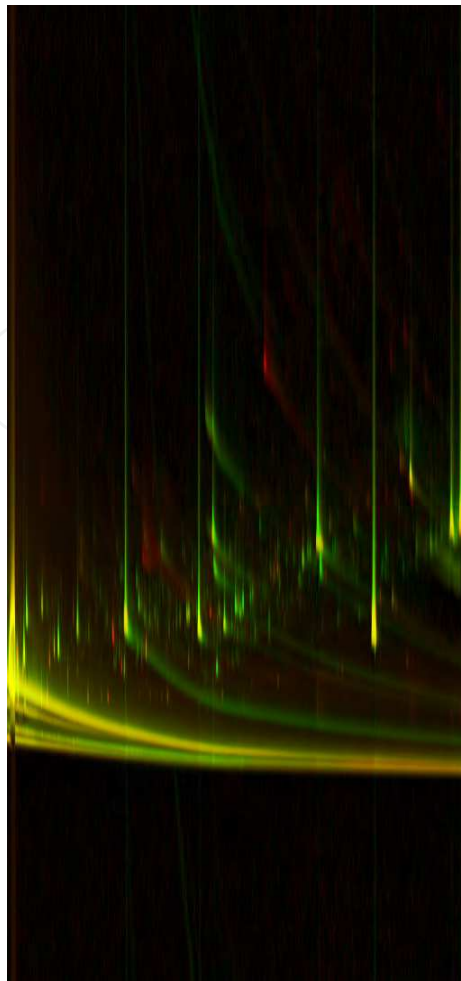
(b) Differential plot of the two Standard-Mix1-1 and Standard-Mix1-2. The plot shows a surplus in Standard-Mix1-1, which is highlighted in green and yellow.
