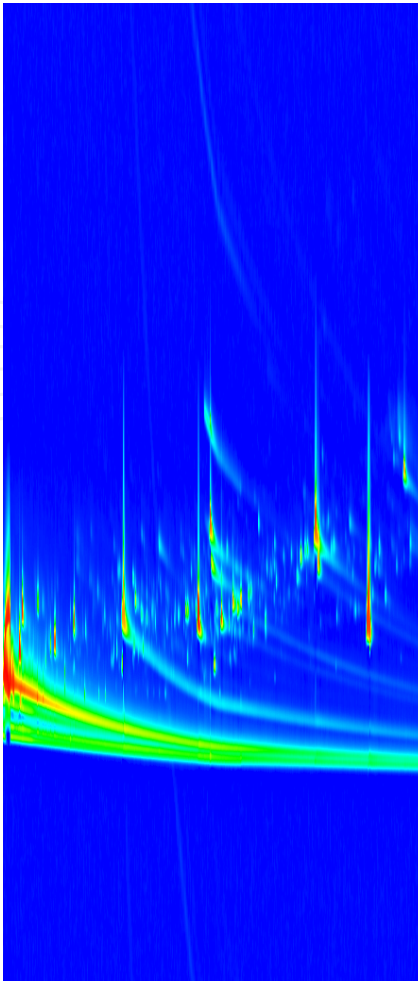
(b) 2D-TIC plot after application of filters. A moving average with window size 3 for smoothing of high frequency noise and a top hat filter for peak removal in order to reduce false positives.
