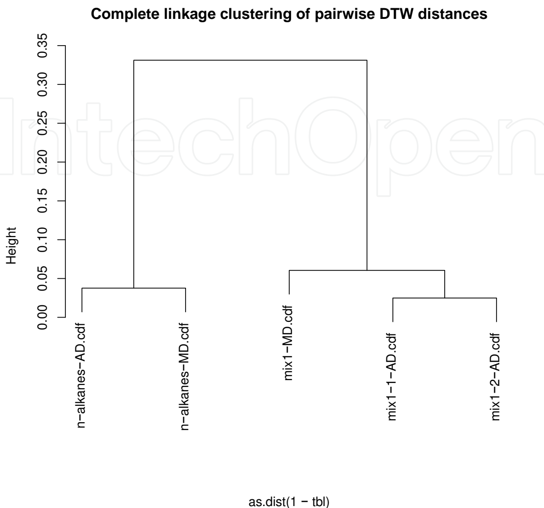
Fig. 3. Clustering of GC-MS samples based on pairwise DTW similarities transformed to distances. The samples are clearly separated into two clusters, one containing the n-alkane standard samples, the other one containing the mix1 samples.
