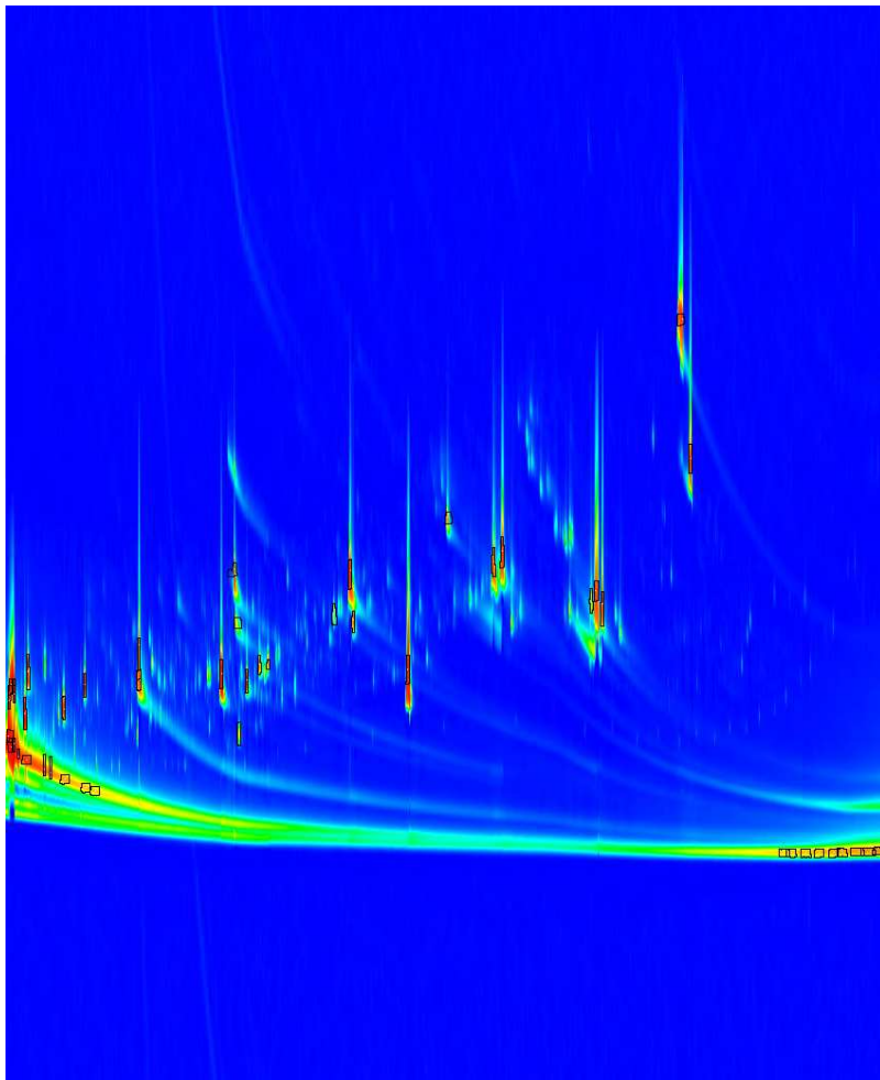
(a) 2D-TIC plot of Standard-Mix1-1 after peak finding and integration with seeded region growing based on the cosine mass spectral similarity with a fusion threshold of 0.99. Peak areas were limited to contain at most 100 points.
