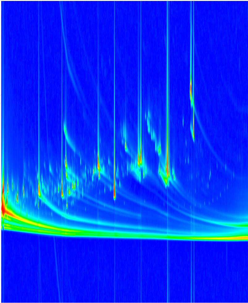
(a) 2D-TIC plot before filters were applied. Long tailing peaks are visible within the vertical dimension. Additionally, high frequency noise is present in the raw exported data, which is barely visible at this resolution.
