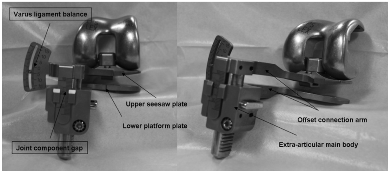
Fig. 1. Offset type tensor
