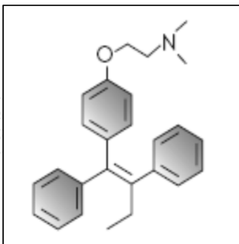
Fig. 3. Chemical structure of tamoxifen.
