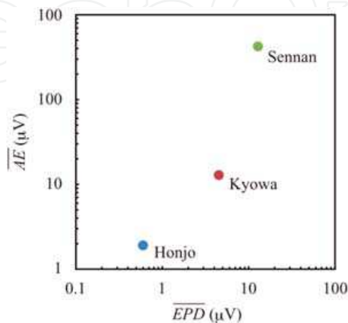
Fig. 13. Positive relation between the average of the earth potential difference ( \overline{EPD} ) and the average of the atmospheric electricity ( \overline{AE} ). Modified from Okubo et al. (2004)
