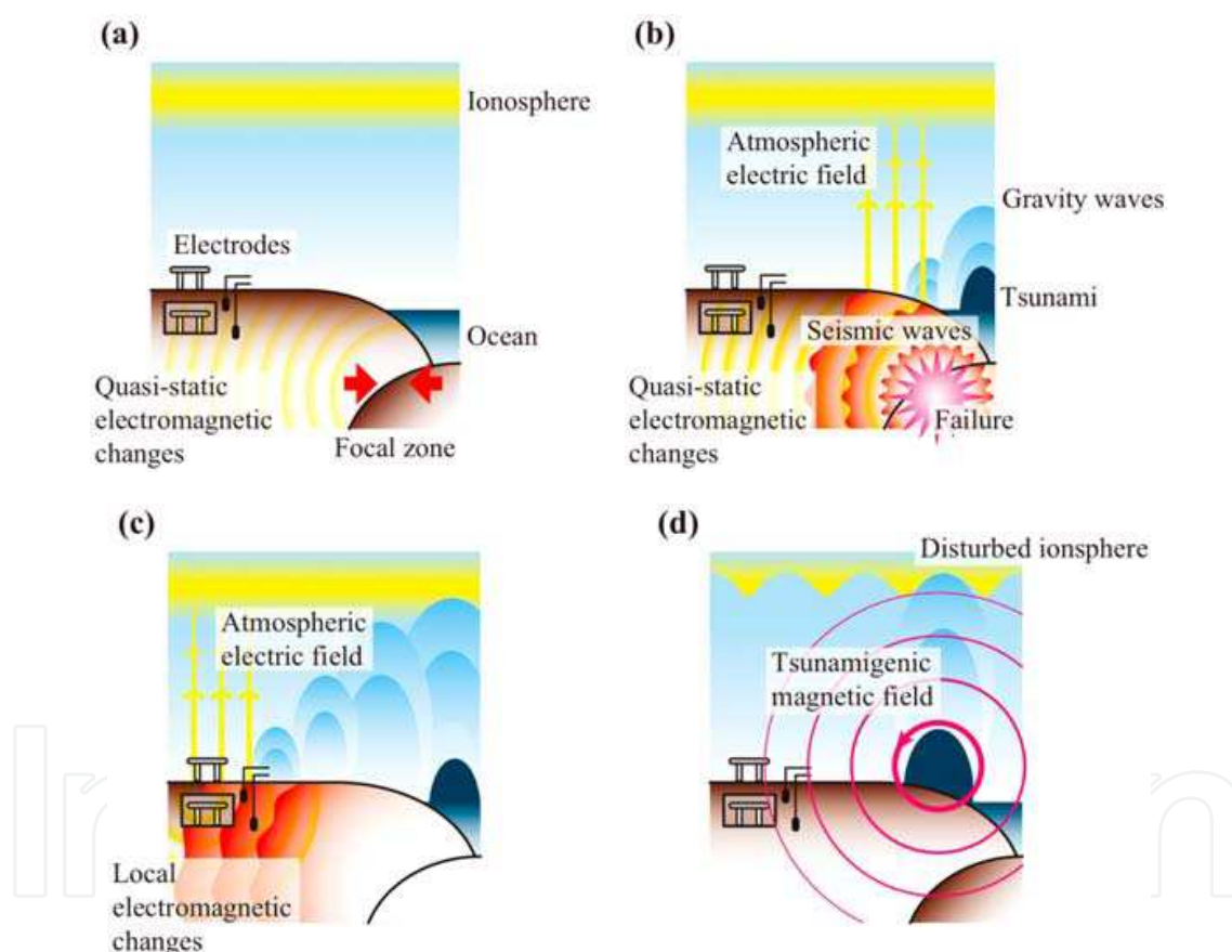
Fig. 19. Electric and electromagnetic phenomena classified in four stages before and after the occurrence of earthquakes: (a) Preseismic, (b) Co-faulting, (c) Coseismic, and (d) Postseismic
