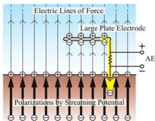
Fig. 17. Generation mechanism of the atmospheric electricity (AE) signals coupled with generation of streaming potential in the near-surface soil layer. Modified from Okubo et al. (2004)
