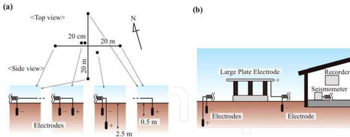
Fig. 8. (a) Observation system of (A) Aobayama site in the early stage. (b) System in the late stage. Modified from Takeuchi et al. (1995, 2000)
