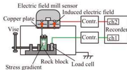
Fig. 4. Setup of non-uniform loading tests using rock blocks. Modified from Takeuchi et al. (2010)
