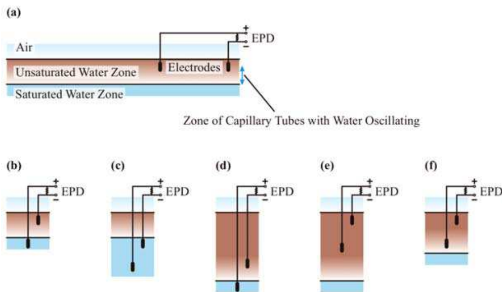
Fig. 18. Six cases of locations with the electrode pair buried and the saturated/unsaturated water zone levels. (a) Both electrodes are horizontally parallel to each other in the unsaturated water zone. (b) One electrode is in the unsaturated water zone; another is in the saturated water zone. (c) Both electrodes are in the saturated water zone. (d) One electrode is deeply situated in the unsaturated water zone; another is deeply situated in the saturated water zone. (e) Both electrodes are in the unsaturated water zone far from the deep saturated water zone. (f) One electrode is in the unsaturated water zone; another is near the saturated water zone. Modified from Okubo et al. (2005)
