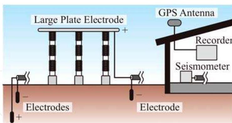
Fig. 10. Observation system of (E) Honjo, (F) Kyowa, and (G) Sennan sites. The seismometer was set up only at (G) Sennan site. Modified from Okubo et al. (2004)
