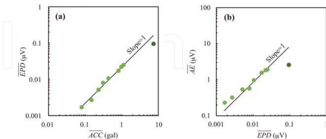
Fig. 15. (a) Positive relation between the average of the earth potential difference ( \overline{EPD} ) and the average of the ground up-down acceleration ( \overline{ACC} ). (b) Positive relation between the average of the atmospheric electricity ( \overline{AE} ) and \overline{EPD} . Linear lines with the slope of 1 are obtained from the plots, excluding the dark plots. Modified from Okubo et al. (2007)
