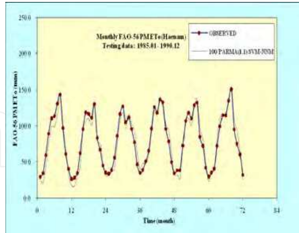
(b) FAO-56 PM ET_0 (100 year)
