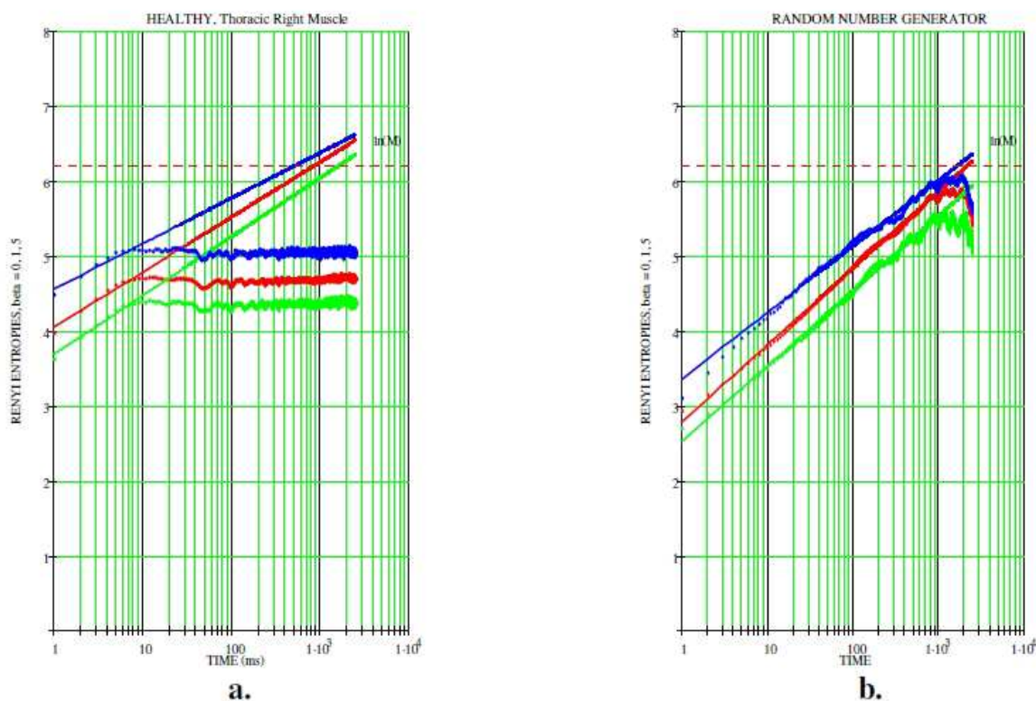
Fig. 1. Entropy vs. \ln t . Top curve \beta = 0 , middle curve \beta = 1 , bottom curve \beta = 5 . a. Subject without LBP for the right thoracic erector spinae muscle; b. Random number generator.
