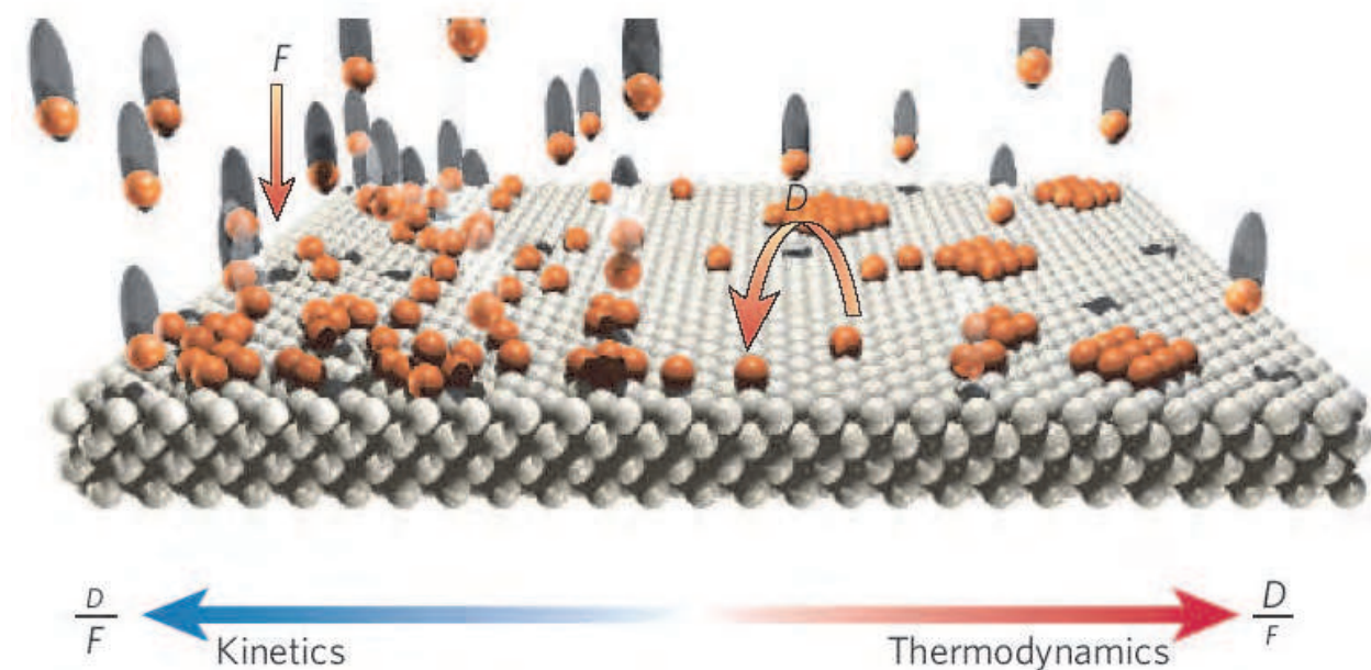
Fig. 10. Atomic-scale view of growth processes at surfaces. The kind of assembled structures is chiefly determined by the D/F diffusivity-to-flux ratio: a small D compared with F favours the aggregation in structures such as metal nanoislands, the reverse situation drives the reaction towards the global energy minimum and is the most suitable for supramolecular assembly (reprinted with permission from J. V. Barth et al., Nature 437, 671 (2005). Copyright 2005 Macmillan Publishers Ltd.)
