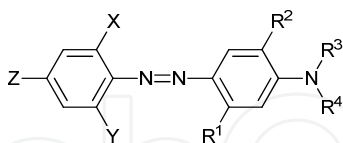
Fig. 4. General structure of aminoazobenzene dyes.
