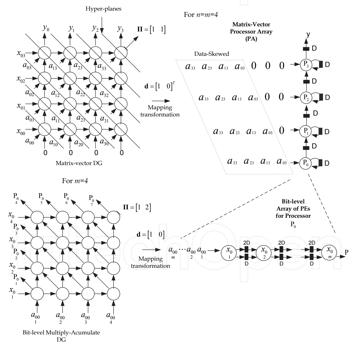
Fig. 2. High-Speed MPPA approach for the reconstructive matrix-vector SP operation
