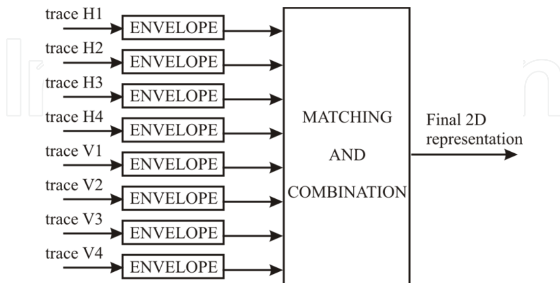
Fig. 1. Functional scheme of the time-domain echo-traces combination technique.
