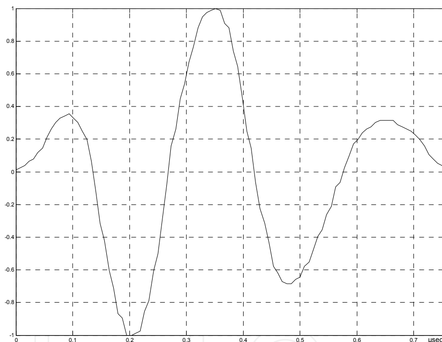
Fig. 5. Ultrasonic echo utilised in type-I experiments.
