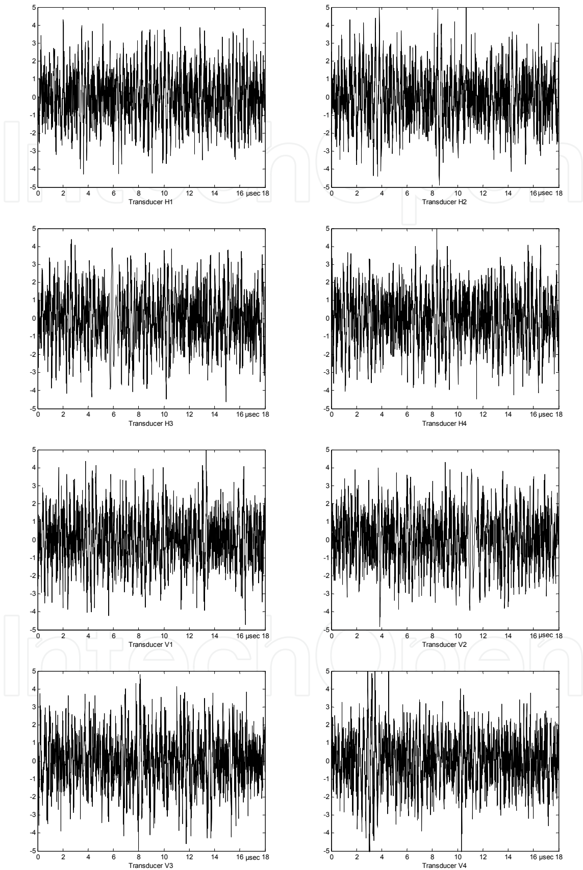
Fig. 7. Ultrasonic traces from the 8 transducers of figure 4 with a simulated SNR_{ini} = 3 dB.
