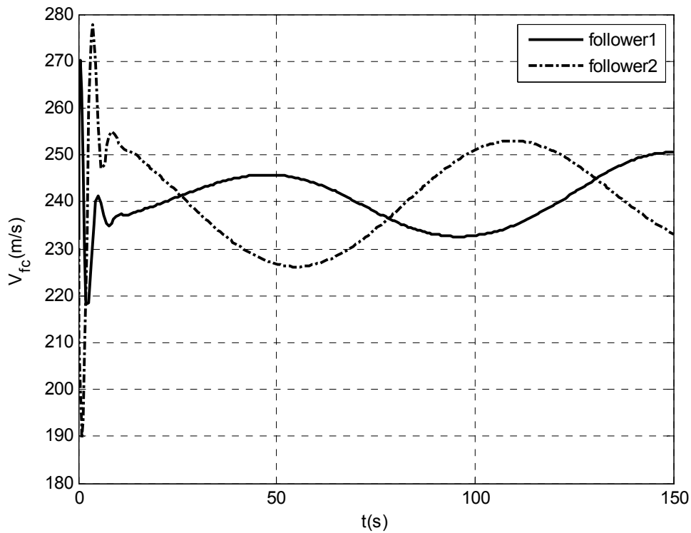
Fig. 16. Velocity commands of followers.
