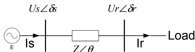
Fig. 6. The equivalent two port network model.
