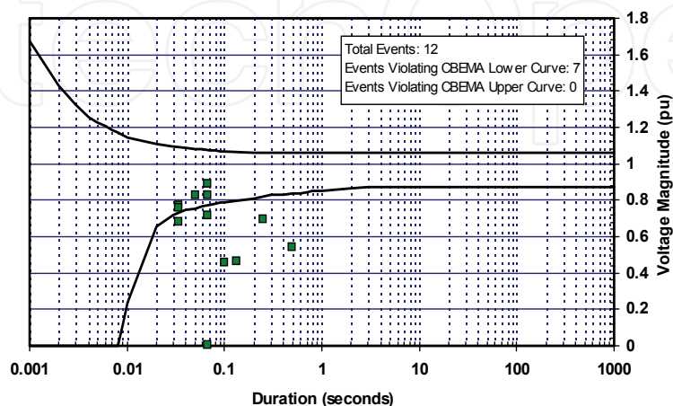
Fig. 1. The CBEMA curve scatter plot
