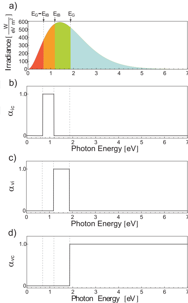
Fig. 4. (a) Radiant emittance of a blackbody at a temperature of 5760 K. Below, plots of the absorption coefficients for (b) IB→CB, (c) VB→IB and (d) VB→CB transitions. The shape of these functions depends on the energy gap and the assumptions made. The depicted forms allow to determine the integral boundaries in equations (12), (13) and (14).
