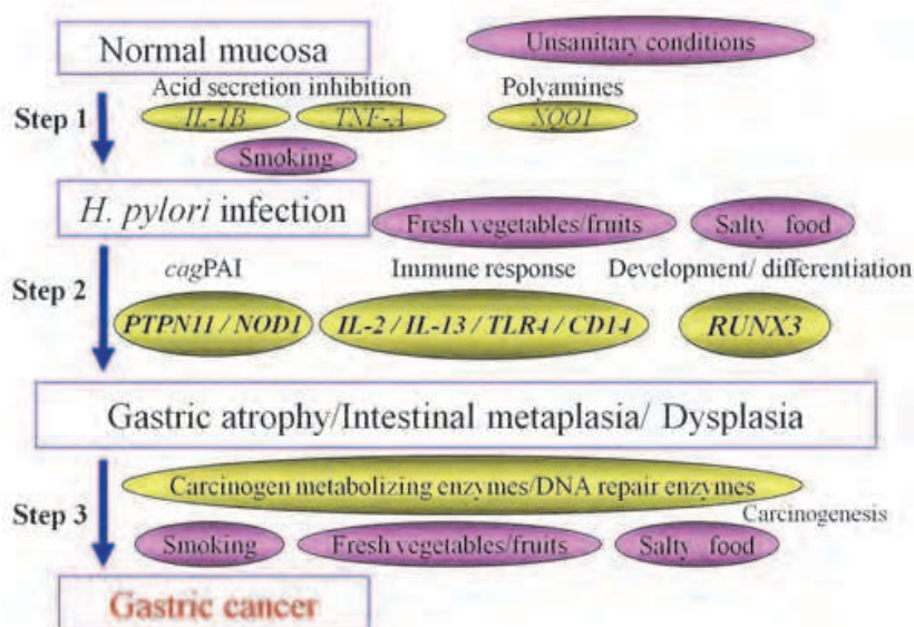
Fig. 1. Steps in Helicobacter pylori -induced gastric cancer.
