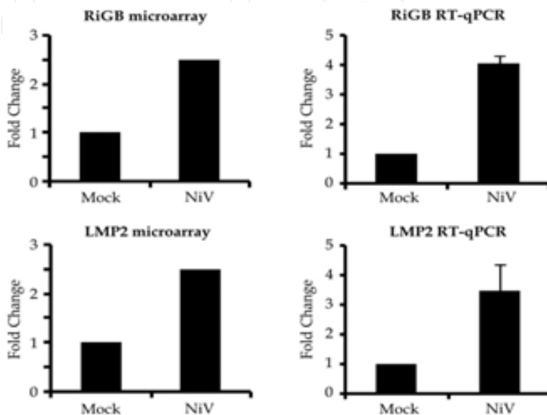
Fig. 6. Example of genes used for the validation of the microarray data. Results obtained from the microarray are shown on the left, whereas RT-qPCR data for the same gene are shown on the right.
