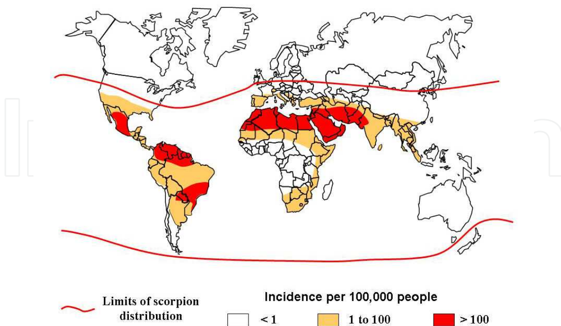
Fig. 3. Scorpionism areas of the world. Reproduced with permission from Chippaux and Goyffon [18].
