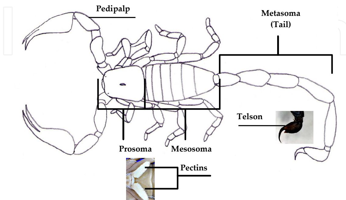
Fig. 2. External appearance of a scorpion's body, showing some anatomic details of Tityus costatus .
