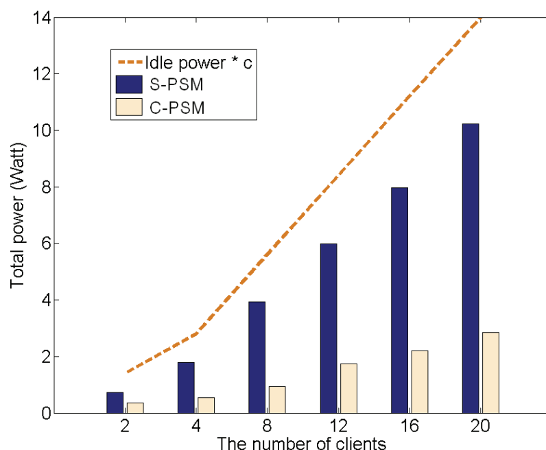
Fig. 5. Total power versus c under the EXP distribution with \delta_j = 10c(\text{ms}) .
