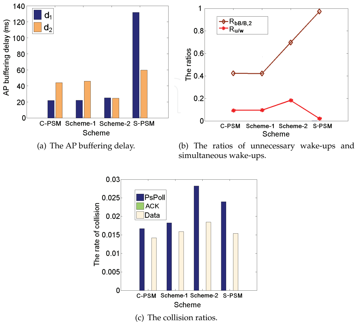
Fig. 4. A comparison of the four schemes under the EXP distribution with \Delta = [15;25]ms .
