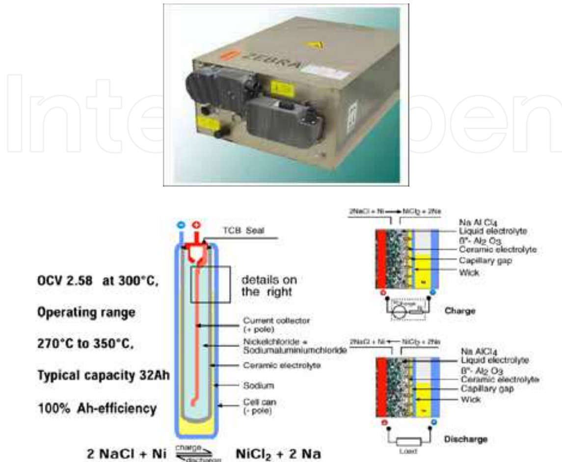
Fig. 5. Zebra battery
