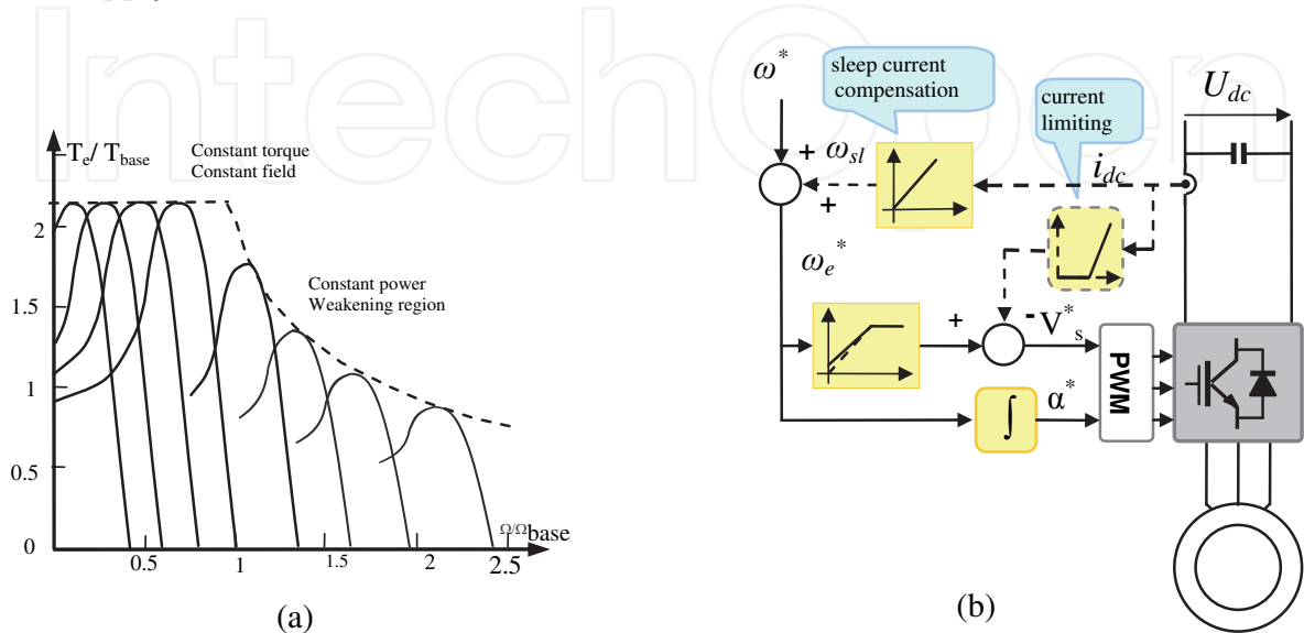
Fig. 9. a. Torque-speed characeristics under V/f control; b. VSI induction motor drive V/f controlled
