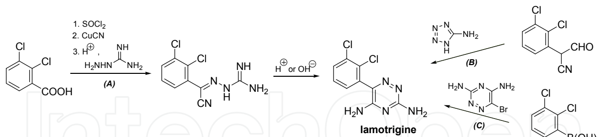
Scheme 16. General methods for the synthesis of lamotrigine.
