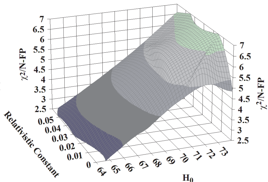
Fig. 4. Calculations of Relativistic Constant A_r from the Simple-DE model with \Omega_m of 0.27.
