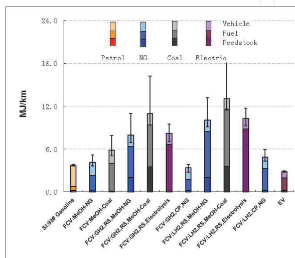
Fig. 3. Comparison of WTW fossil fuel consumptions
