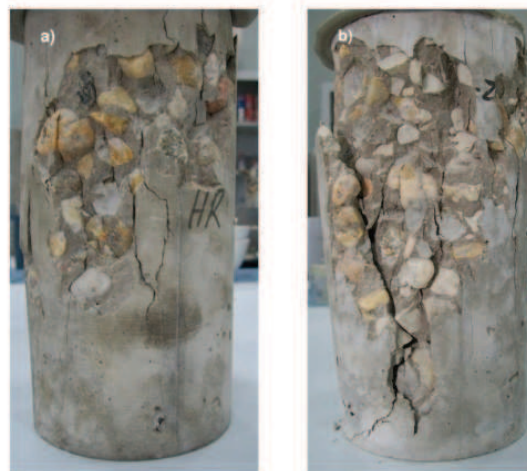
Fig. 3. Types of compressive fracture: a) Concrete CC. b) Recycled concrete RC-25
