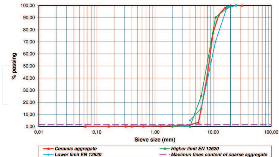
Fig. 1. Particle size grading of ceramic aggregate
