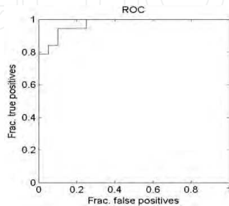
Fig. 12. ROC curve presenting the classification performance of 10 most significant features derived with help of 100 Ridge regression models. AUC is 95%.
