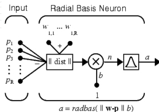
Fig. 1. Radial Basis Function Neural Network.
