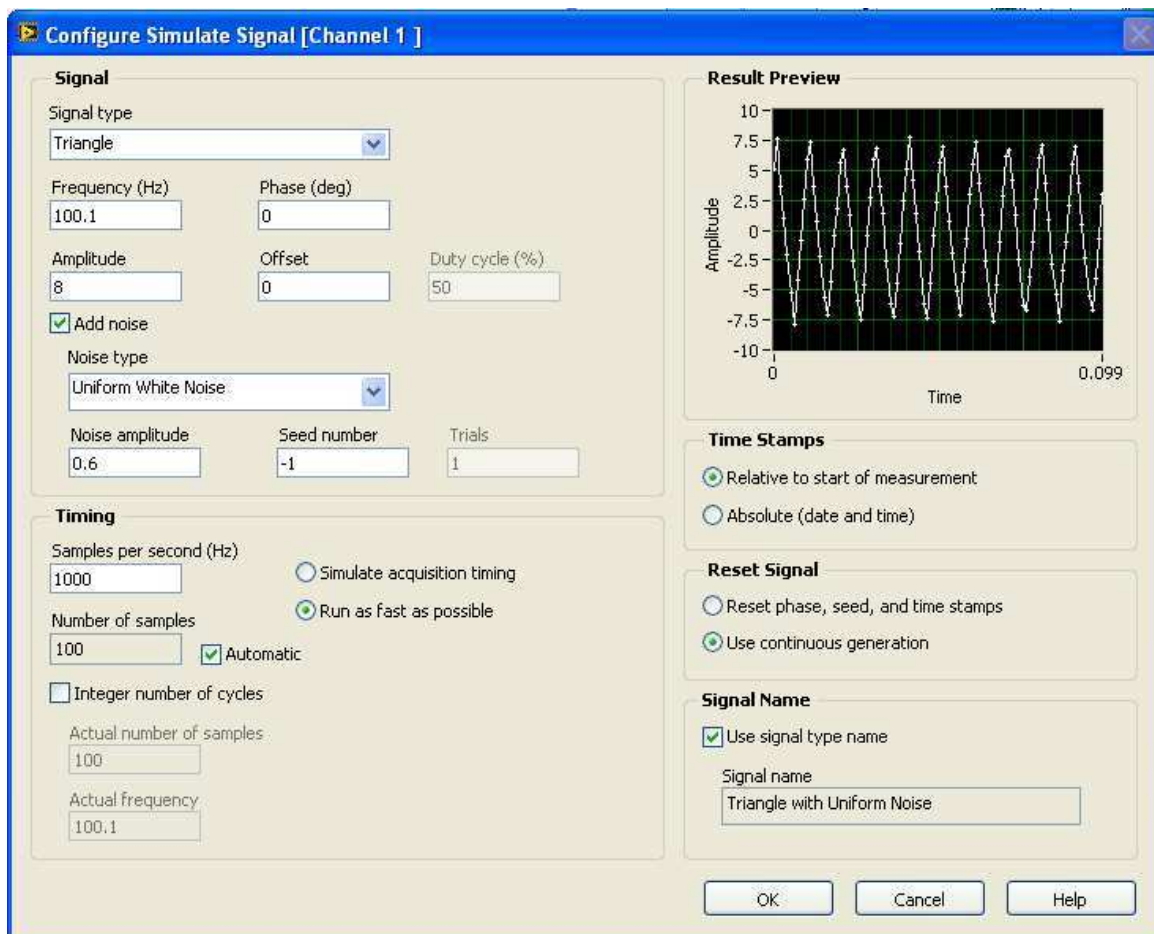
Fig. 13. Simulate signal generator SubVI (a) Icon (b) Dialog box
